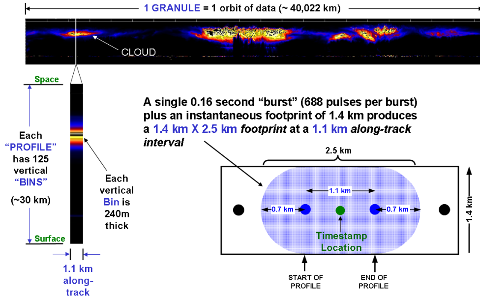
Figure 2. CloudSat Data Footprint and Granule Size
