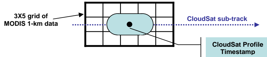
Figure 3. MODIS-AUX footprint compared with a CloudSat profile
