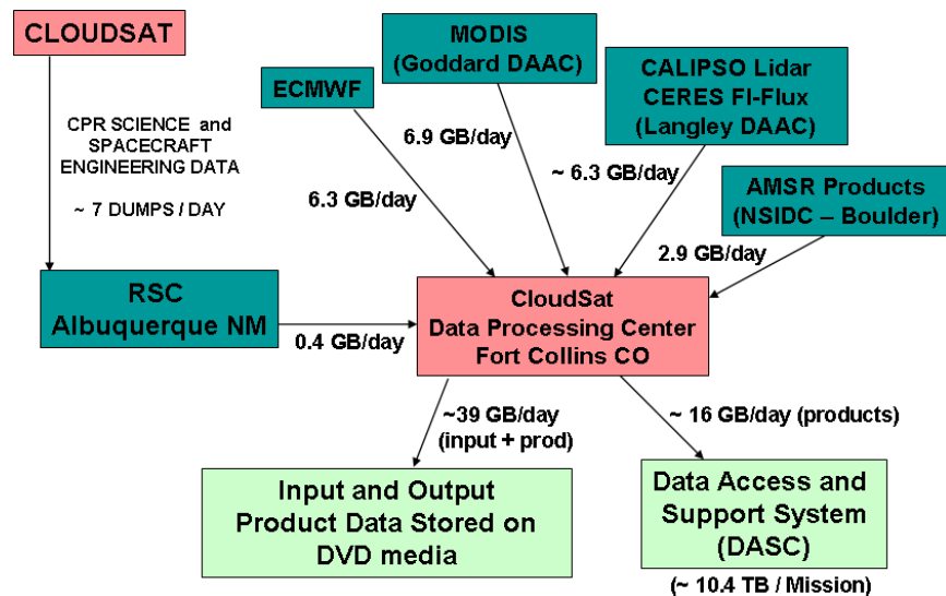
Figure 1. CloudSat System Data Flow
